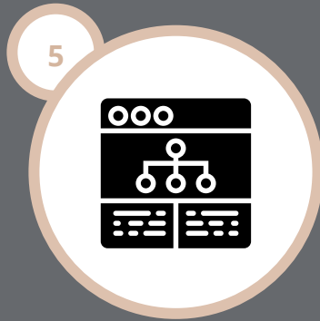
DATA ANALYTICS
